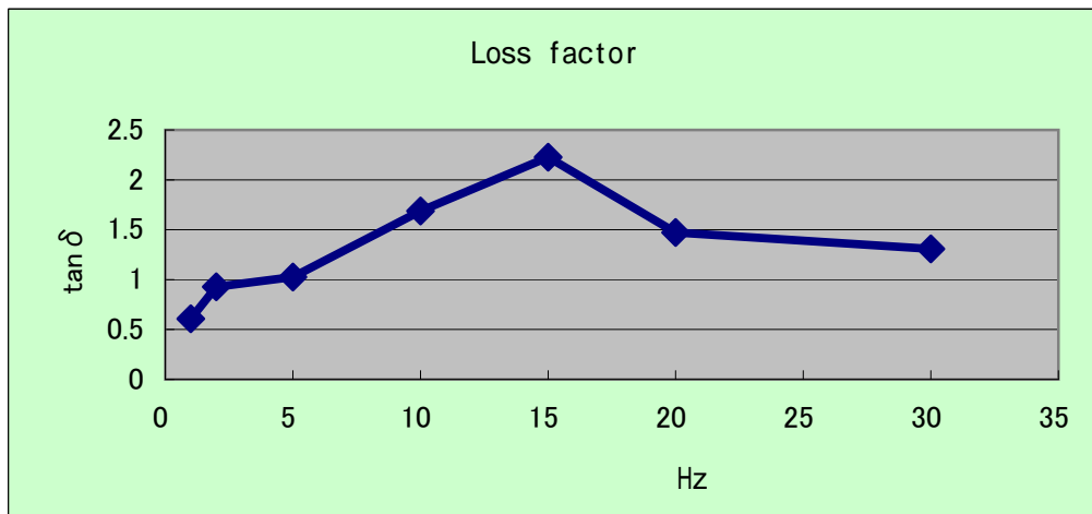
Loss-factor by various frequency
